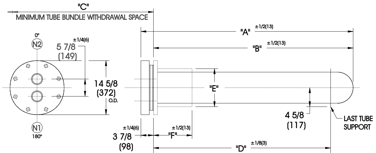
DIMENSIONS SHOWN AS: inches (mm)
