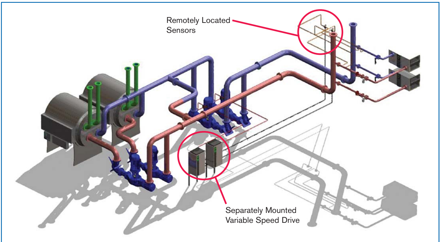
Figure 1 - Typical Primary/Secondary Chilled or Heating Water System Incorporating Variable Speed Drives
