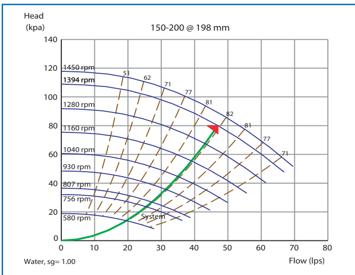
Figure 4 - Constant Curve Control
