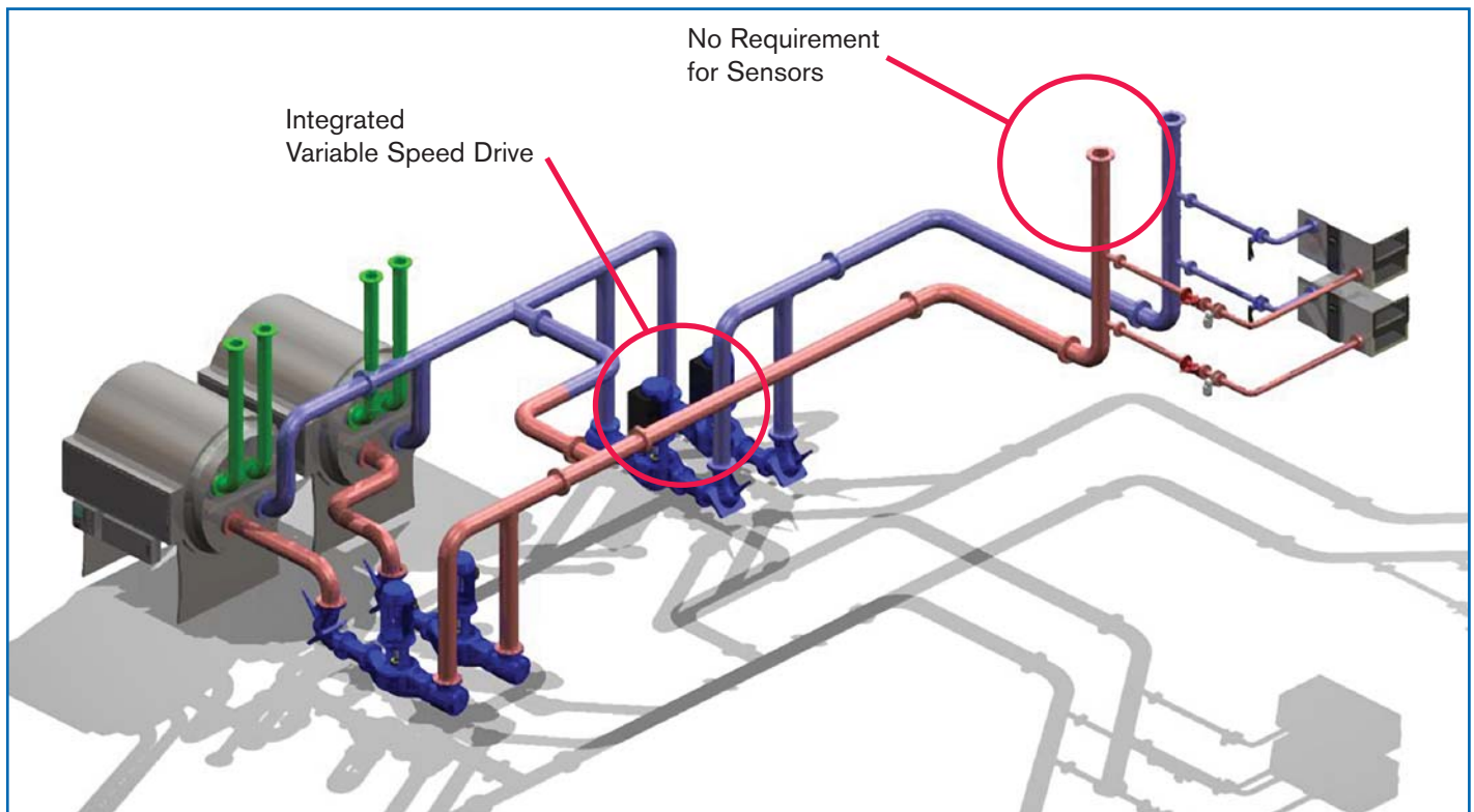
Figure 3 - Primary/Secondary Chilled or Heating Water System Incorporating Armstrong IVS Sensorless Pumps
